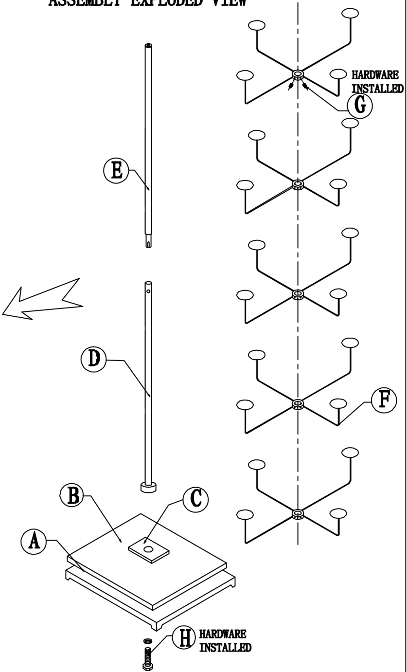
ASSEMBLY EXPLODED VIEW
