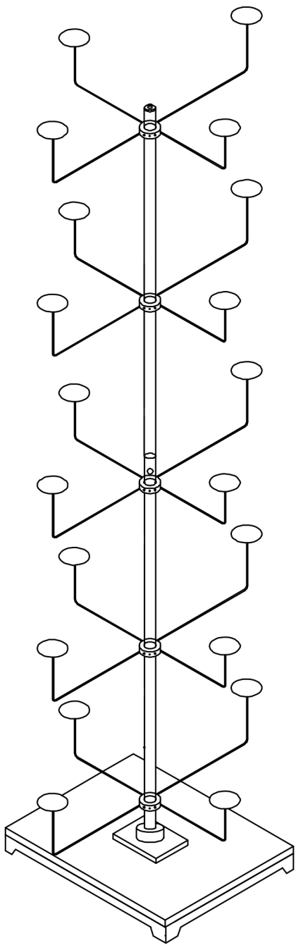
ASSEMBLING DRAWING
