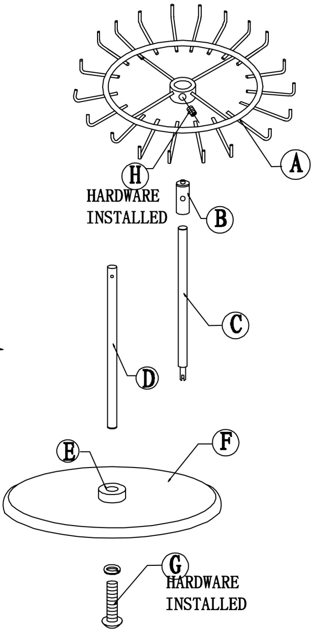
ASSEMBLY EXPLODED VIEW
