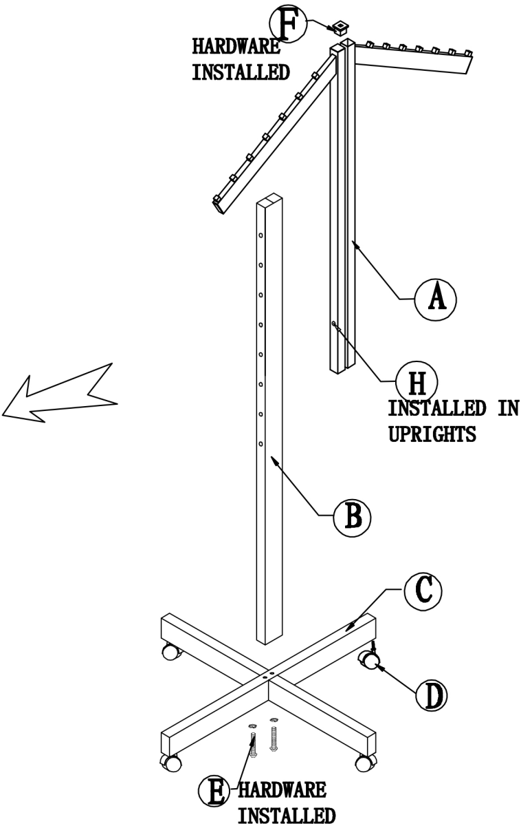
ASSEMBLY EXPLODED VIEW
